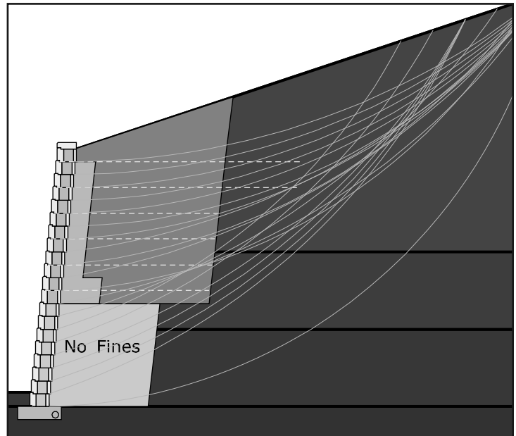
Figure D-8. NFC/Geogrid CCS Section - ICS Analysis
