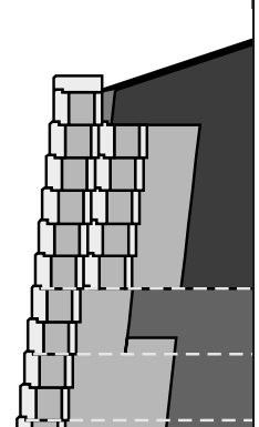
Lower no-fines structure depth cannot be less than 70% of the depth of the Upper Structure
