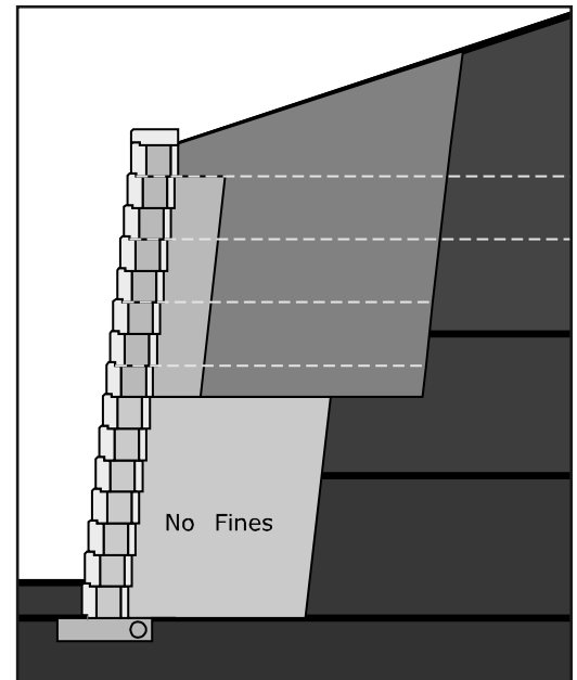
Figure E-2. NFC/Geogrid CCS Section
