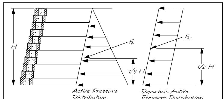
Figure 5-1. Dynamic and Static Active Pressure Distribution
