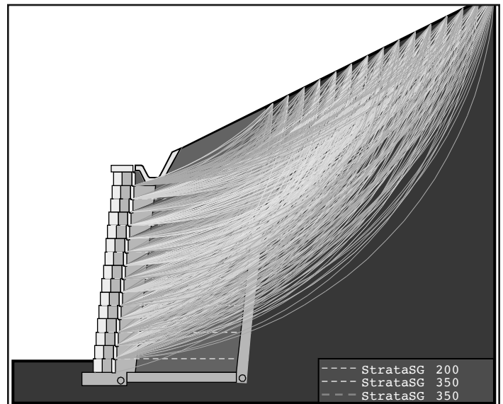
Figure 7-13. ICS Pressure Map Diagram
