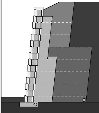
Geogrid lengths in the Upper Structure cannot be less than the standard minimum of 4 ft (120 cm) or 60% of the Upper Structure height
