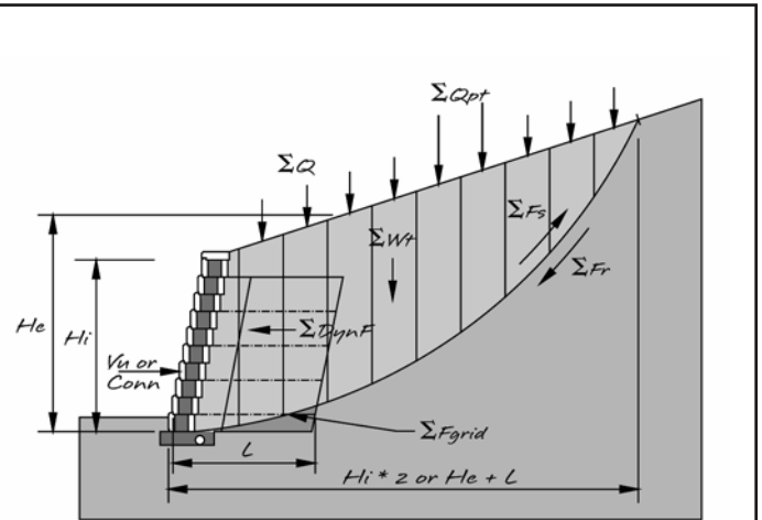
Figure 7-12. ICS Design Envelope & Forces
