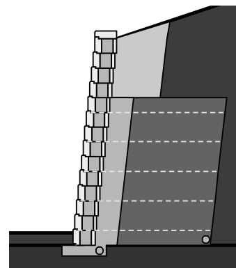
No-fines concrete in the Upper Structure cannot be less than the standard minimum of 2 ft (60 cm) and is commonly designed to be 40% of the Upper Structure height
