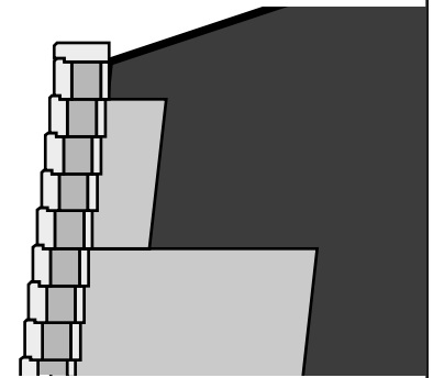
Standard gravity wall above no-fine concrete wall
