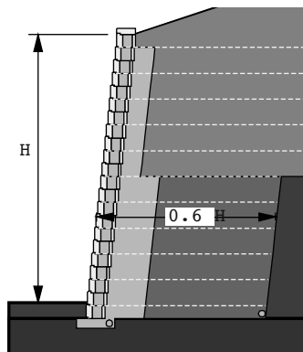
Geogrid lengths in the Lower Structure are recommended to be not less than 60% of the total wall height
