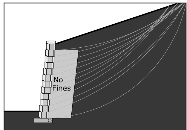
Figure D-6. NFC - ICS Analysis
