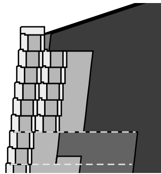
Double block or AB Fieldstone long anchoring unit wall above geogrid wall
